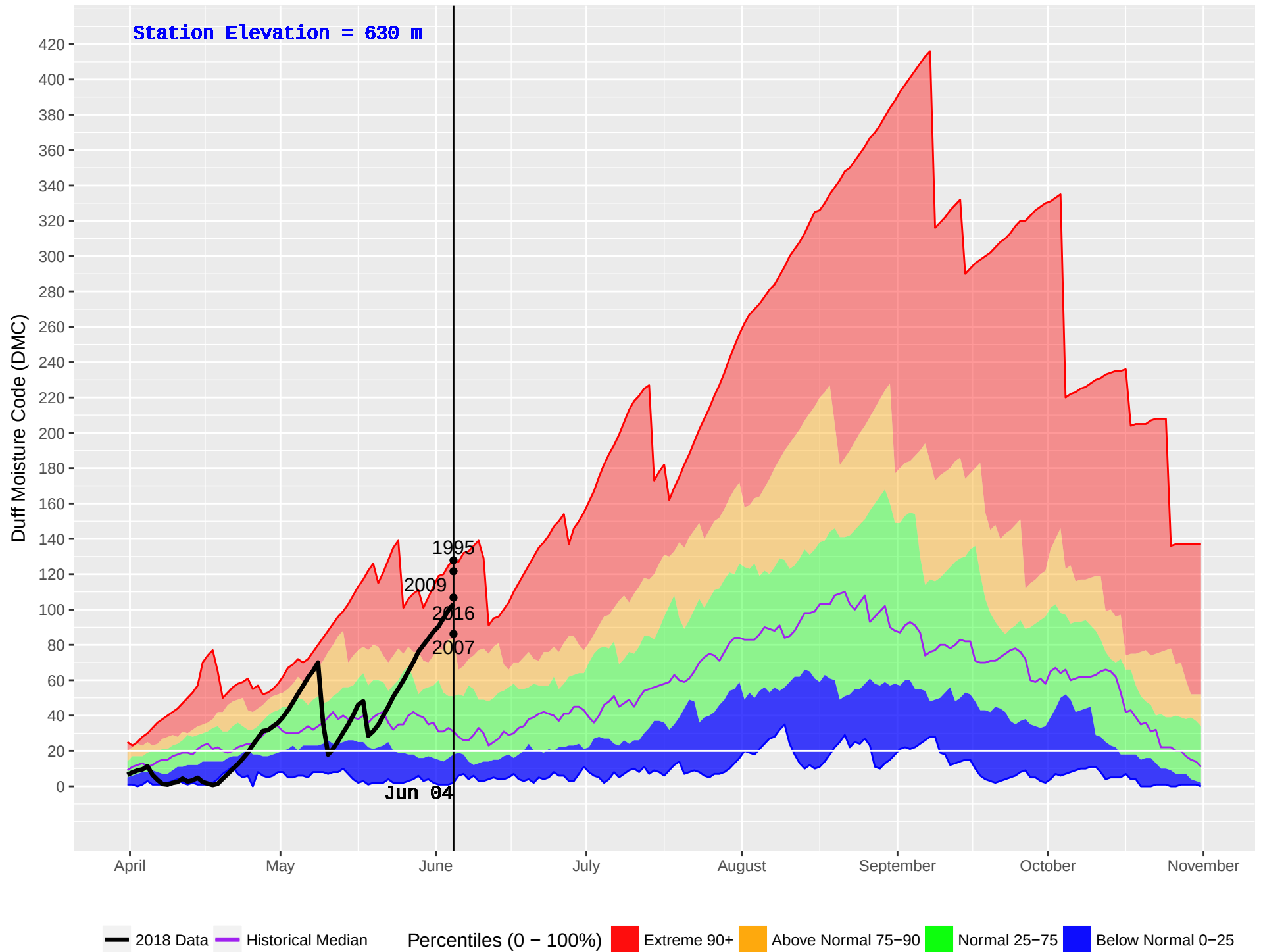
GRAND FORKS (392) : Historical (1981–2016) and Current (2018) Noon Duff Moisture Code (DMC)
