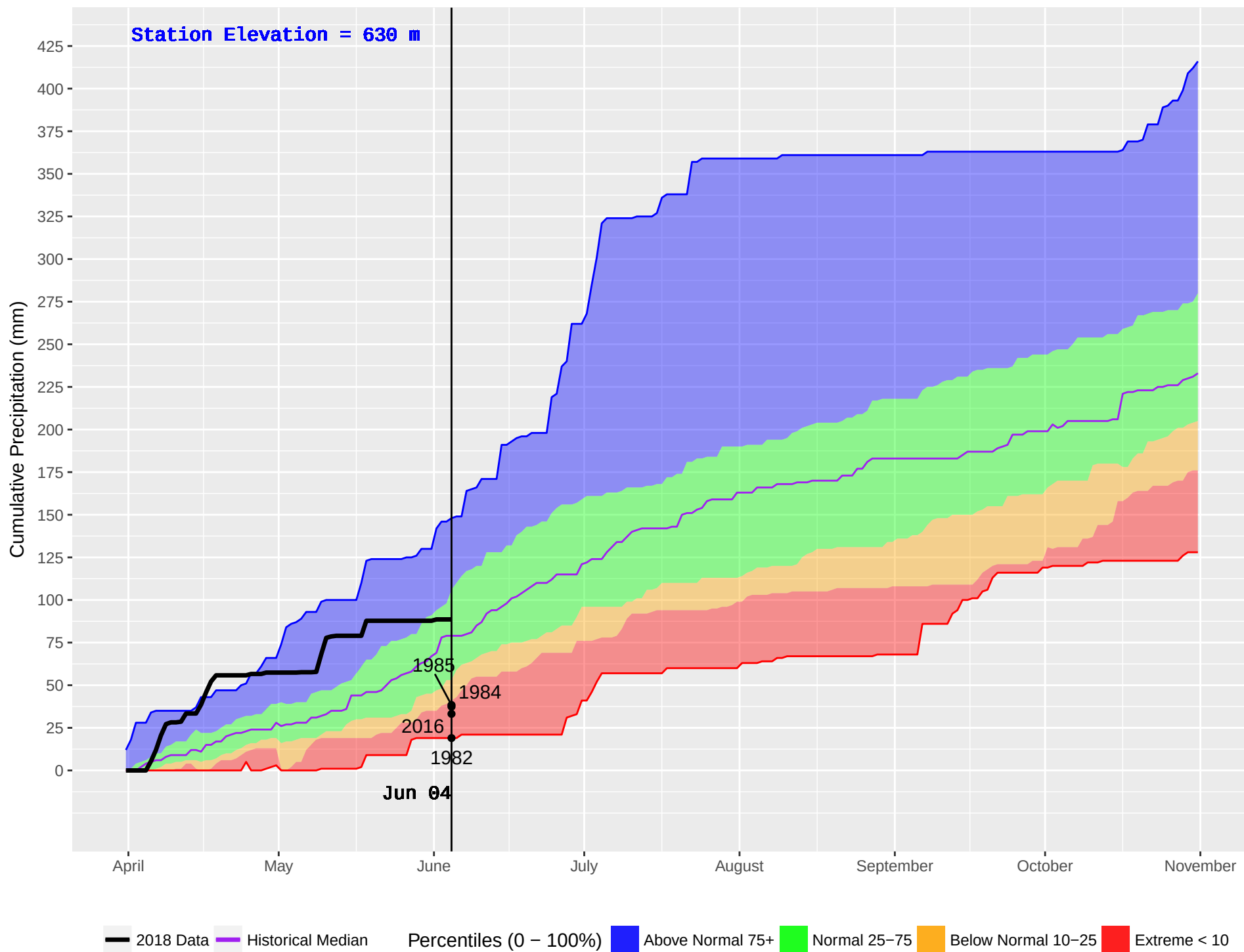
GRAND FORKS (392) : Historical (1981–2016) and Current (2018) Noon Cumulative Precipitation
