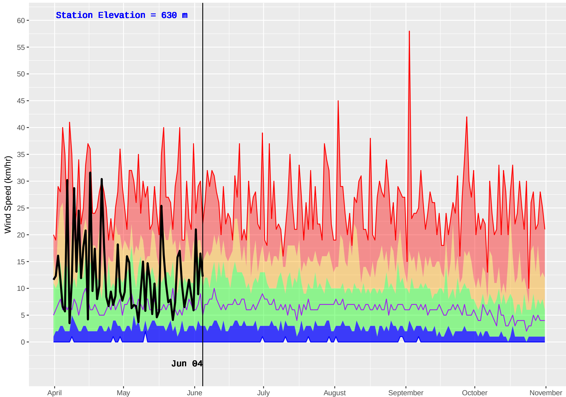
GRAND FORKS (392) : Historical (1981–2016) and Current (2018) Noon Wind Speed
