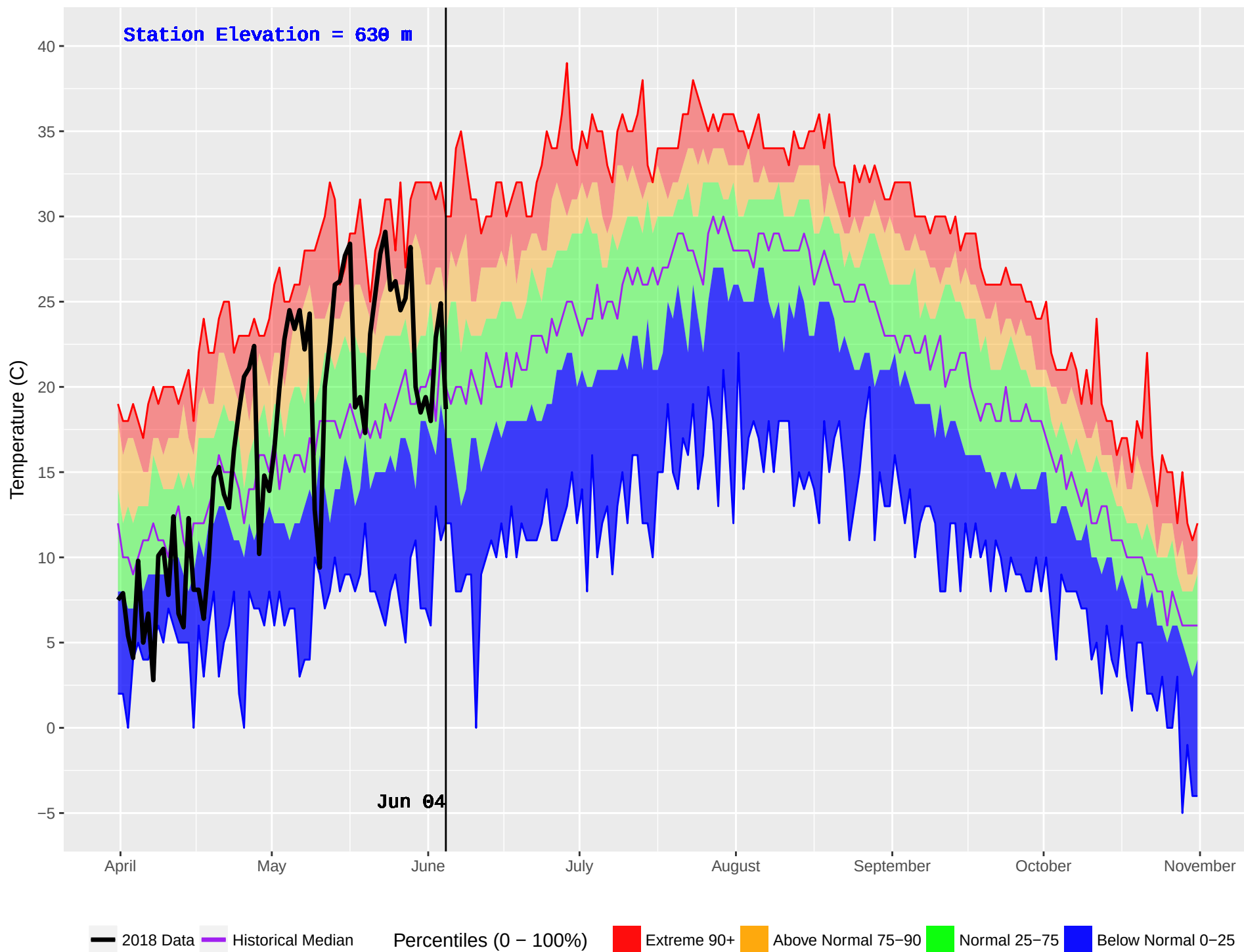
GRAND FORKS (392) : Historical (1981–2016) and Current (2018) Noon Temperature
